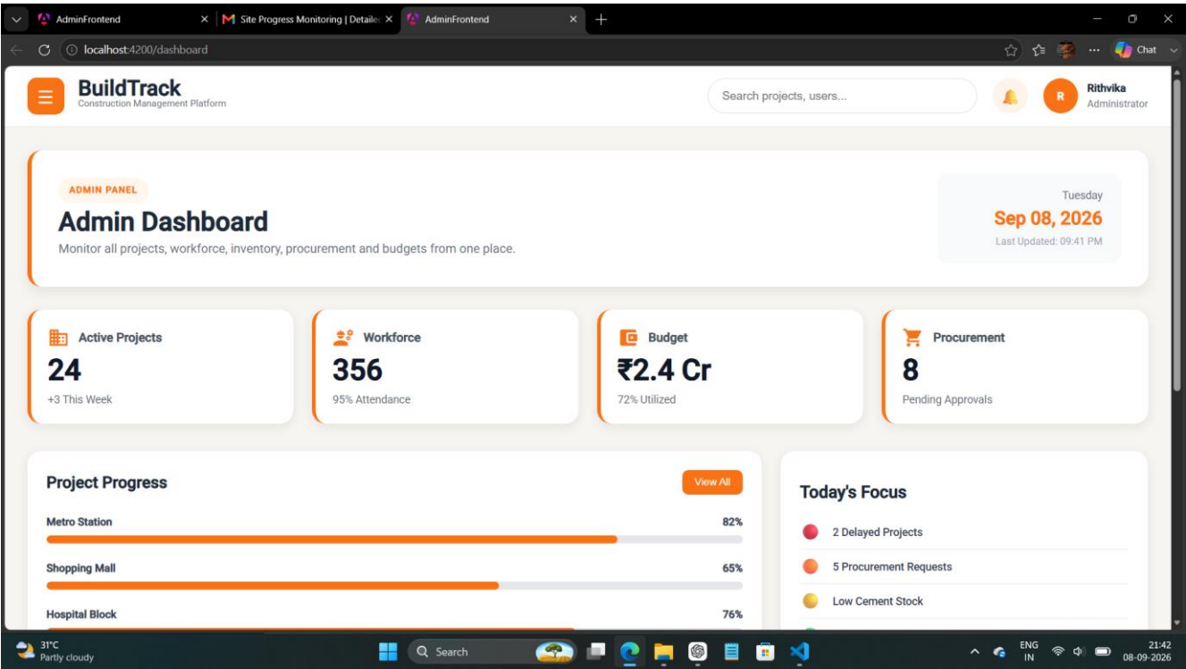
Figure 2: BuildTrack Administrator Dashboard
