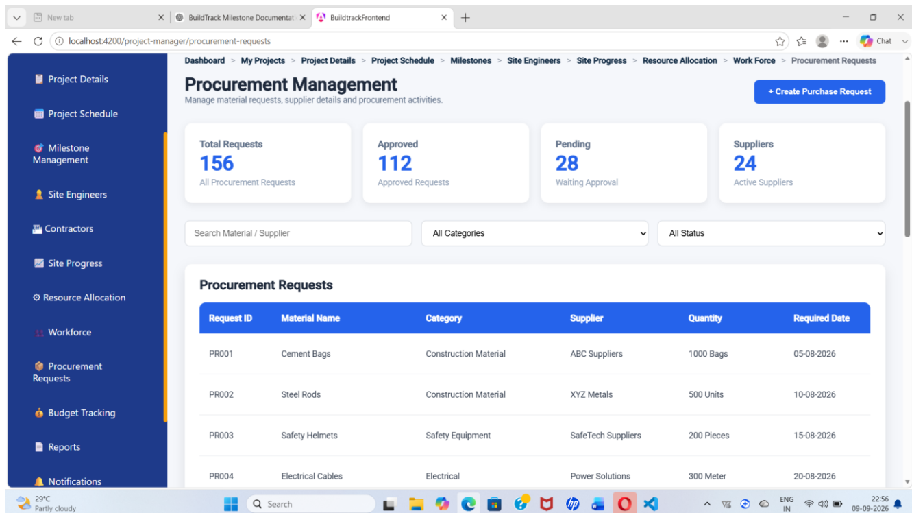
Figure 19: BuildTrack Project Manager – procurement requests
