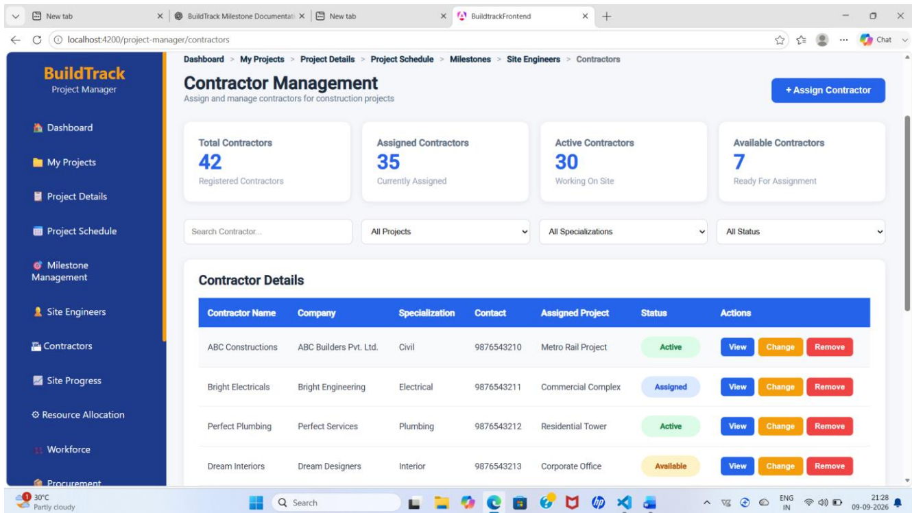
Figure 15: BuildTrack Project Manager – contractors
