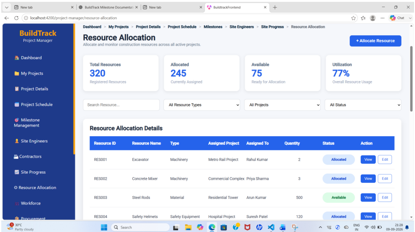
Figure 17: BuildTrack Project Manager – resource allocation
